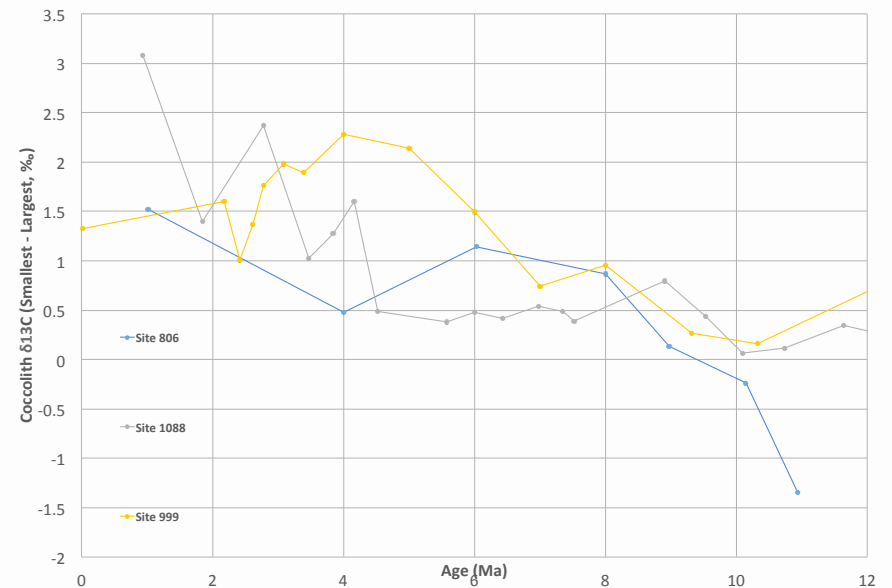
Isotopic difference between large & small cells
