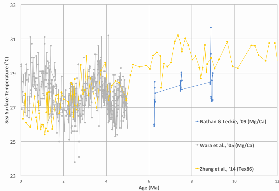
ODP Site 806 Sea surface temperature
