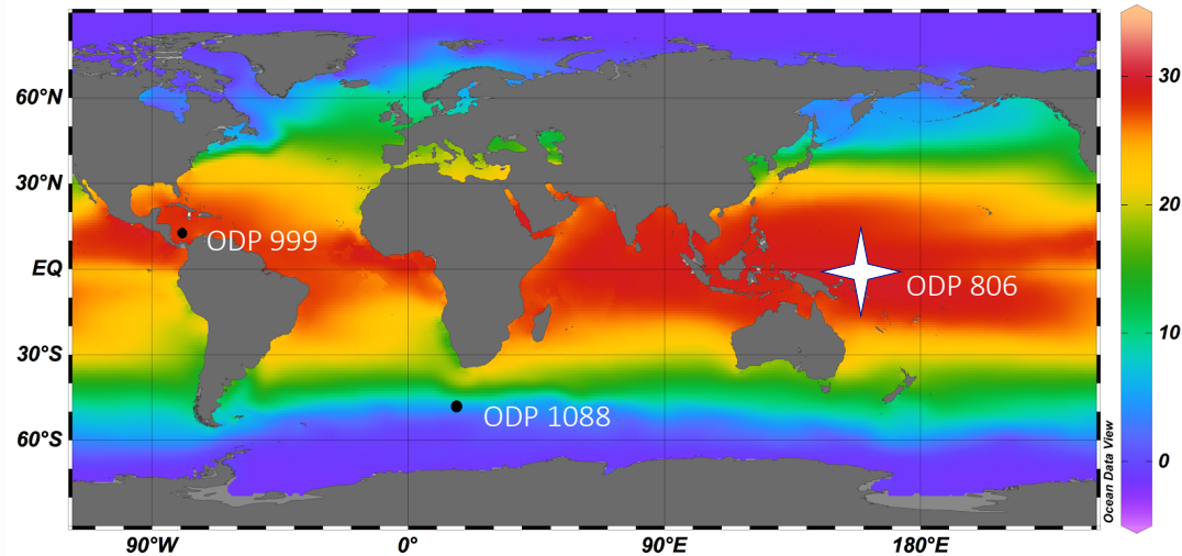
ODP Site 806 Sea surface temperature
