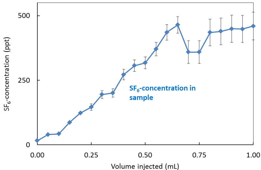
SF 6 injection into flow-loop
