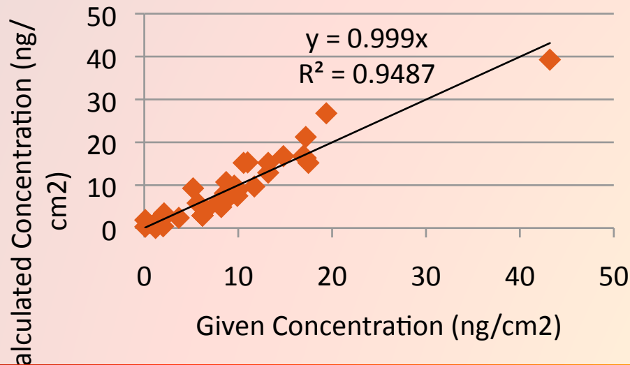
Lead Calculated vs. Given Concentration
